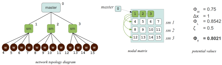
Figure 6: Load balanced topology p = 16, p_{sm} = 3
